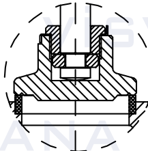
DN 15...DN 80
