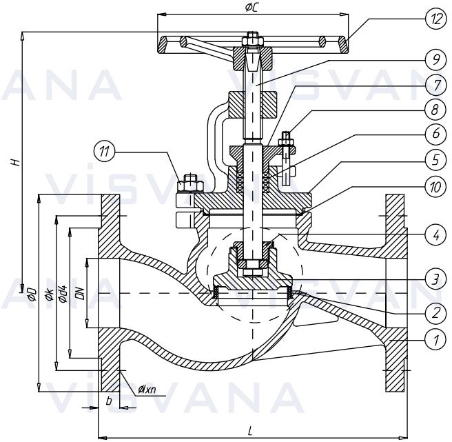
DN 100...DN 350
