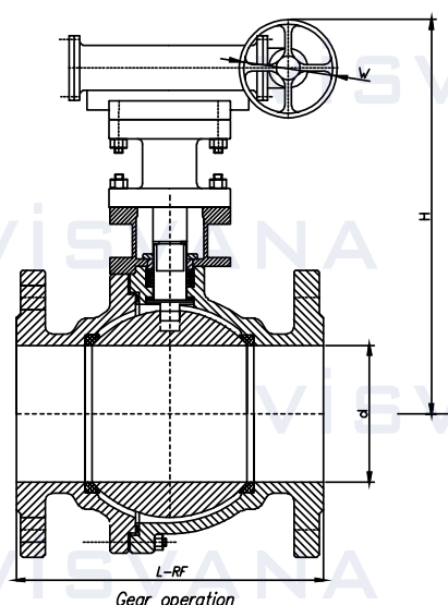
Gear operation
